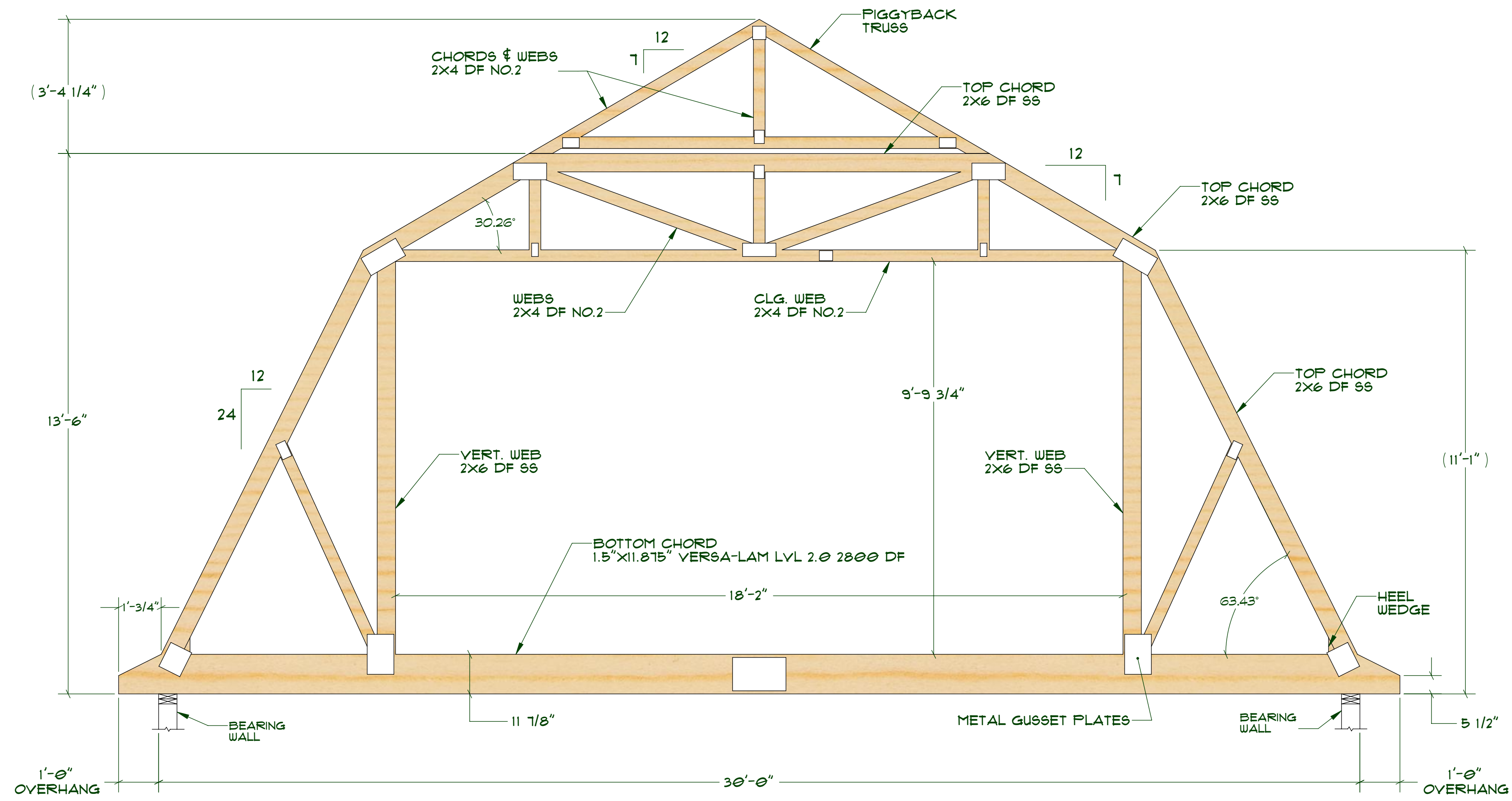
30' GAMBREL ATTIC TRUSS W/ FIGGYBACK
