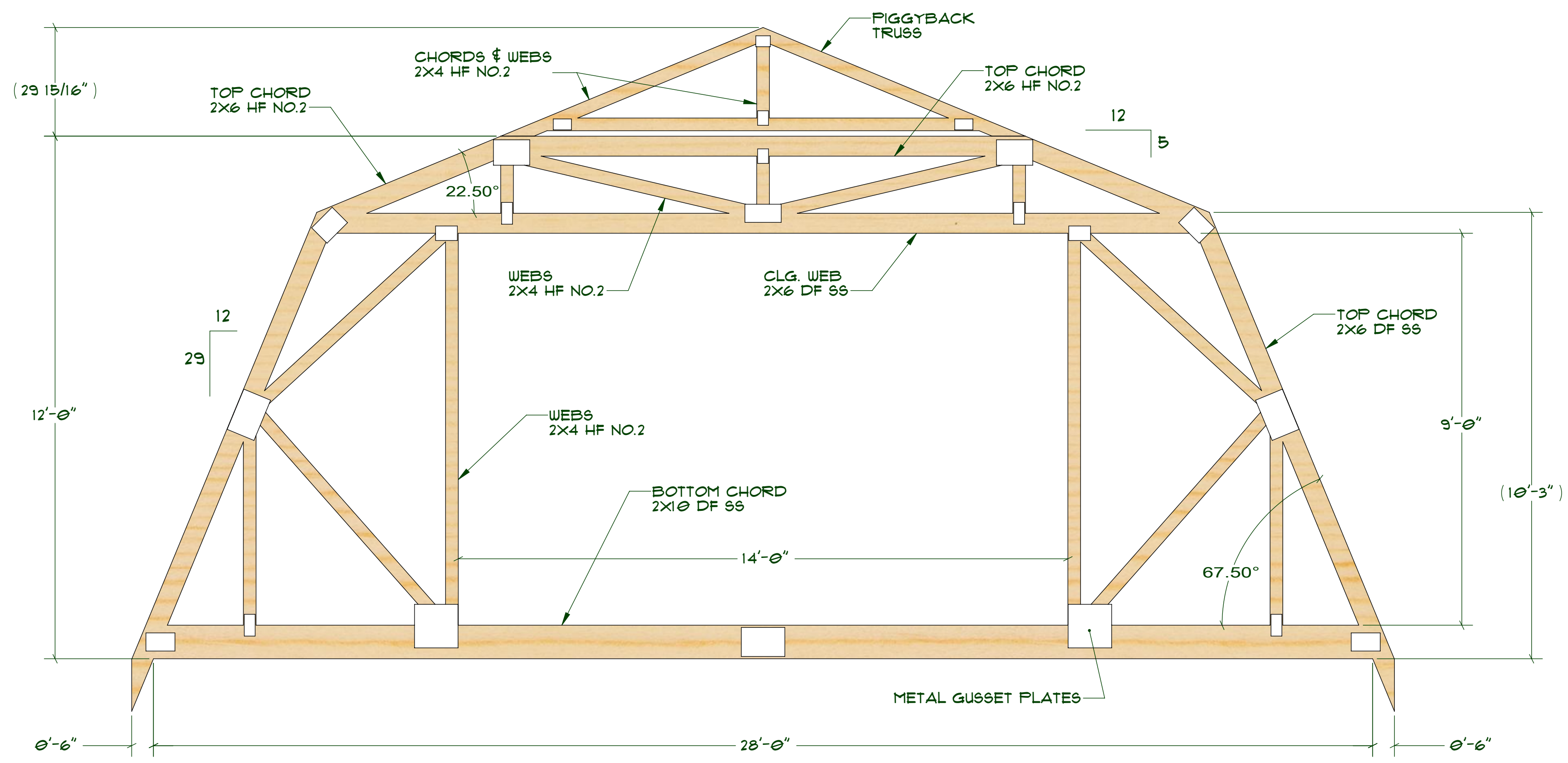
28' GAMBREL ATTIC TRUSS W/ FIGGYBACK
