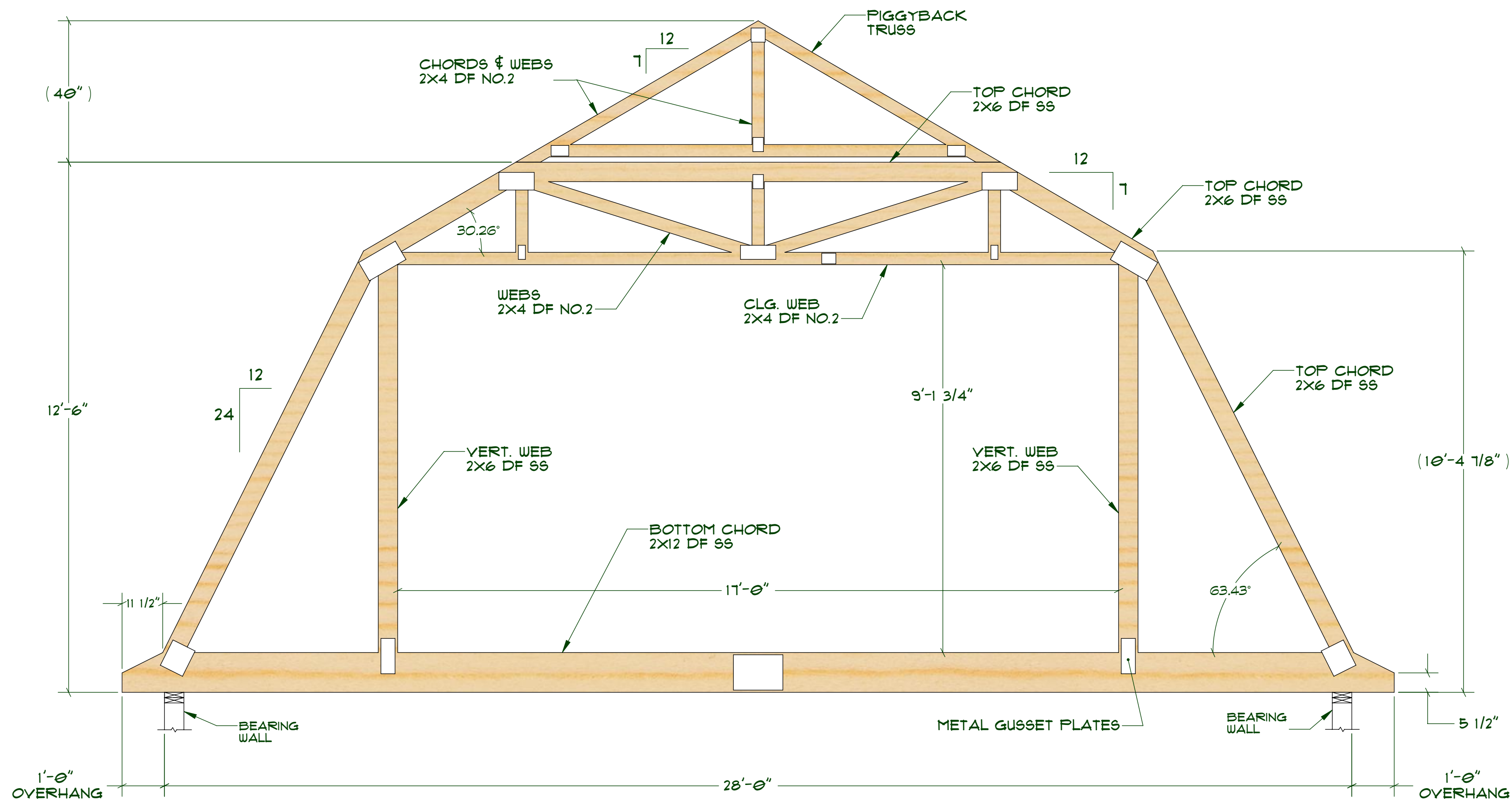
28' GAMBREL ATTIC TRUSS W/ FIGGYBACK
