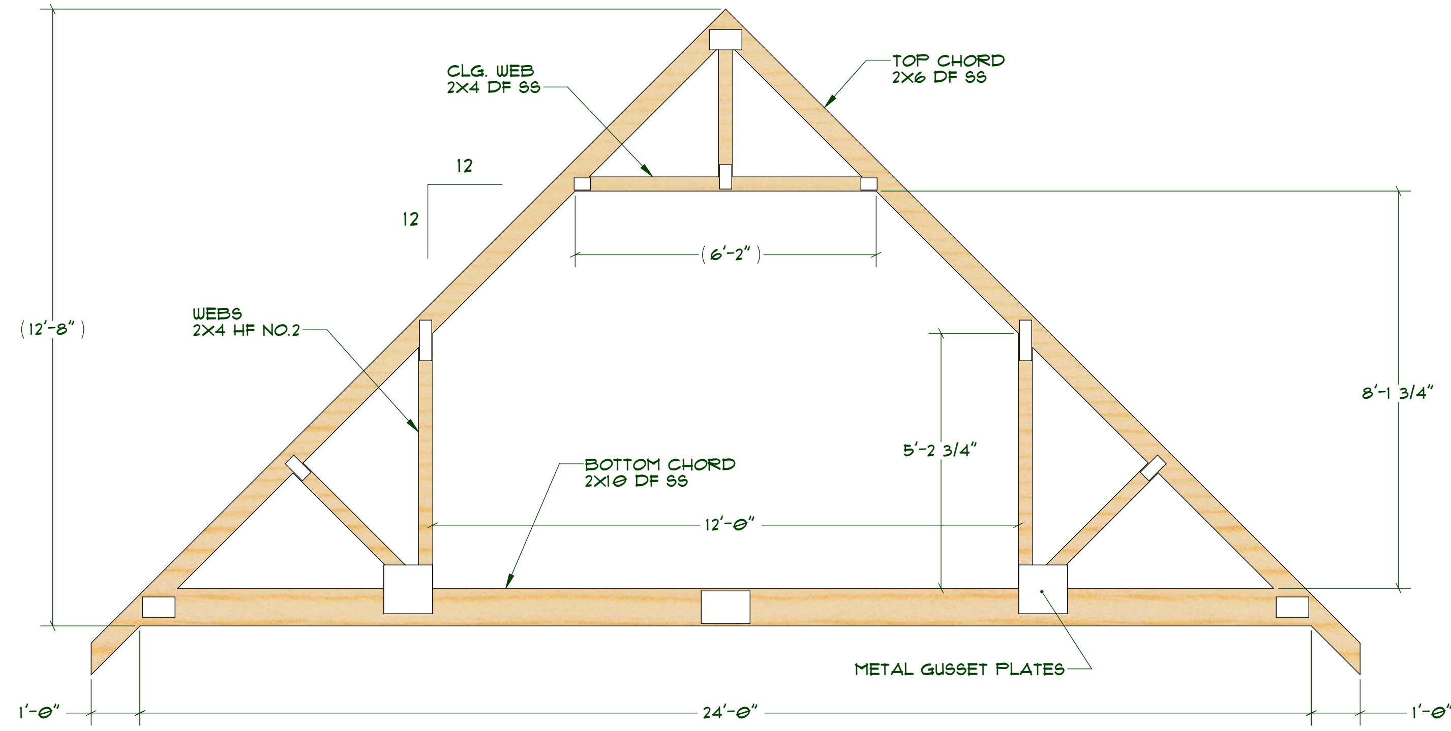
24' ATTIC TRUSS
