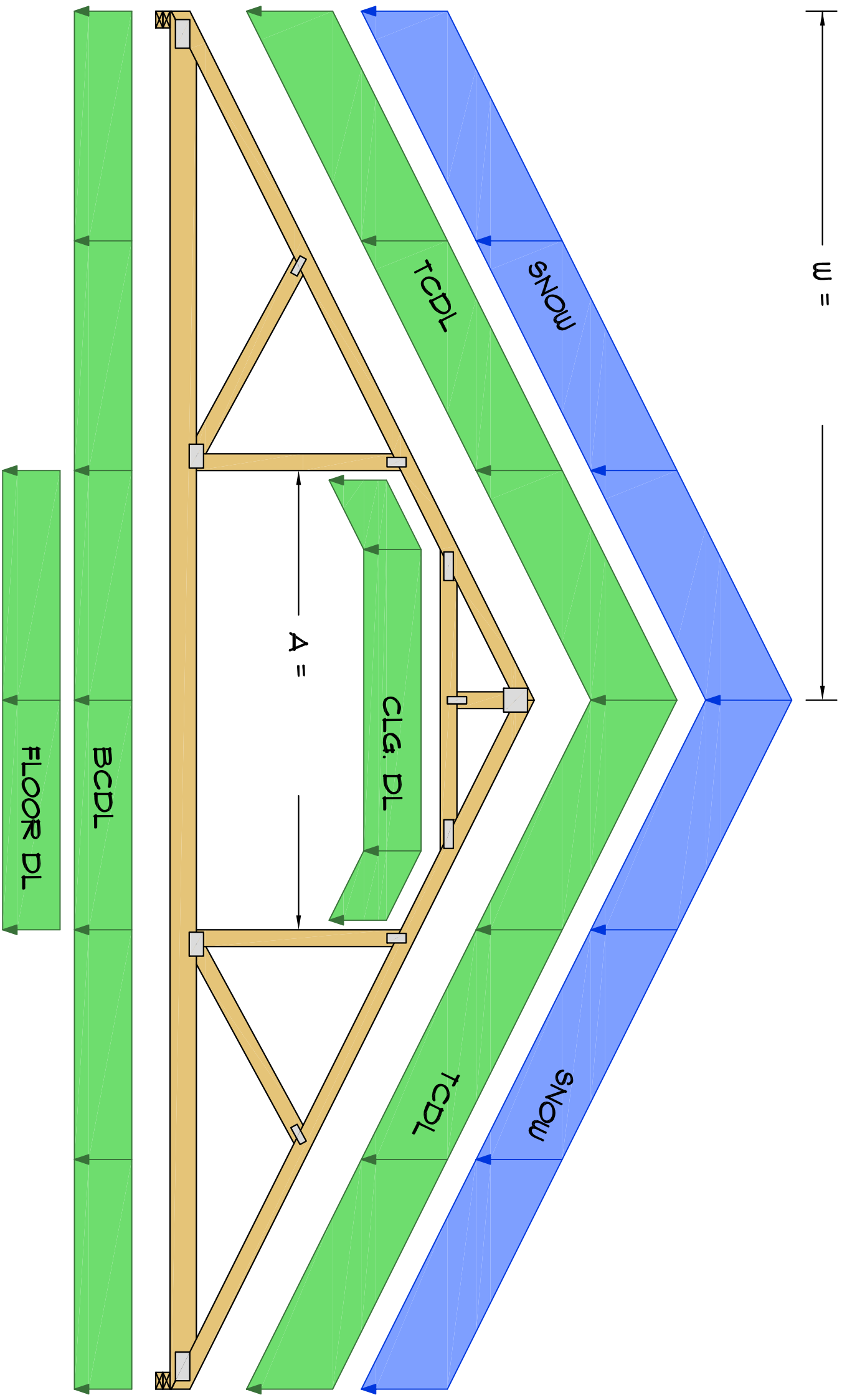
BALANCED SNOW AND DEAD LOADS
