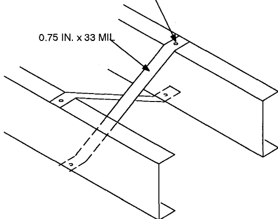
X-BRACING
