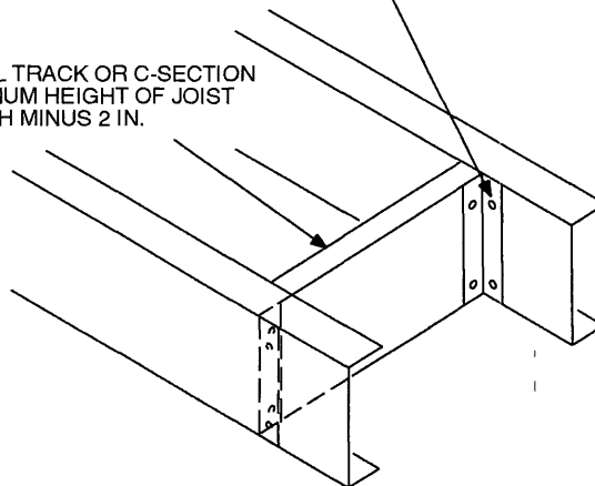
SOLID BLOCKING
