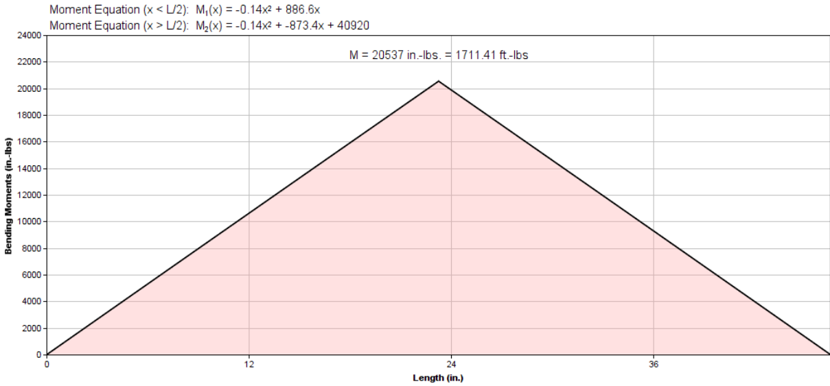
Beam - Moment Diagram
