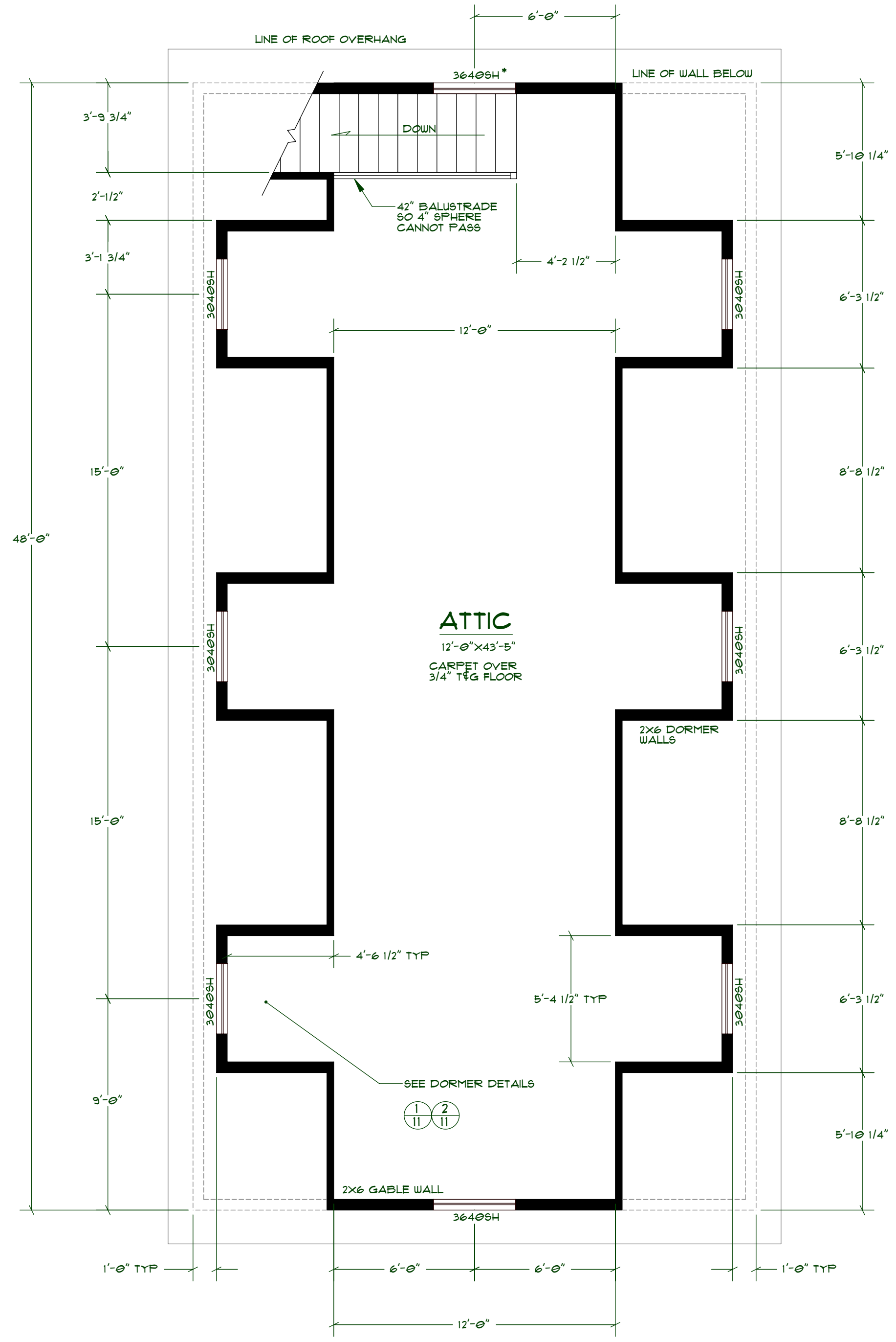
ATTIC FLOOR PLAN
