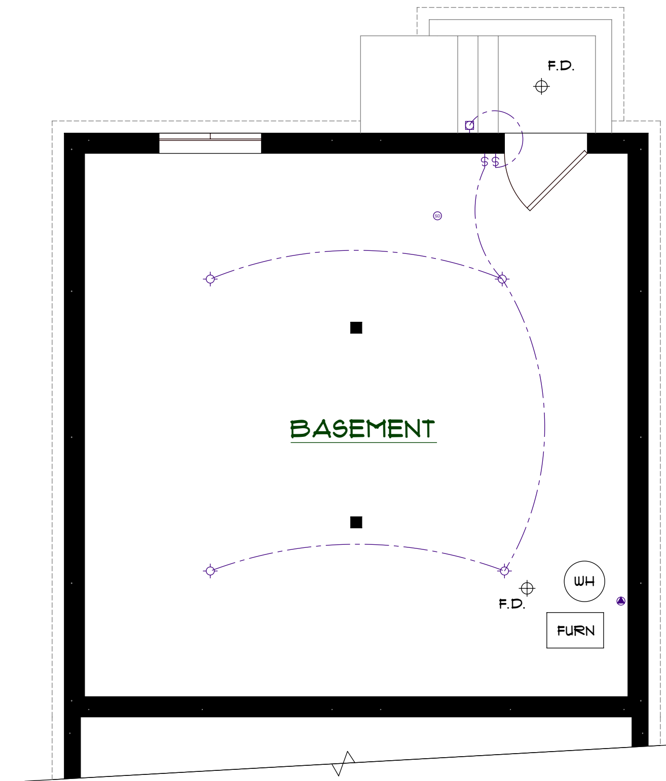
BASEMENT ELECT. PLAN
