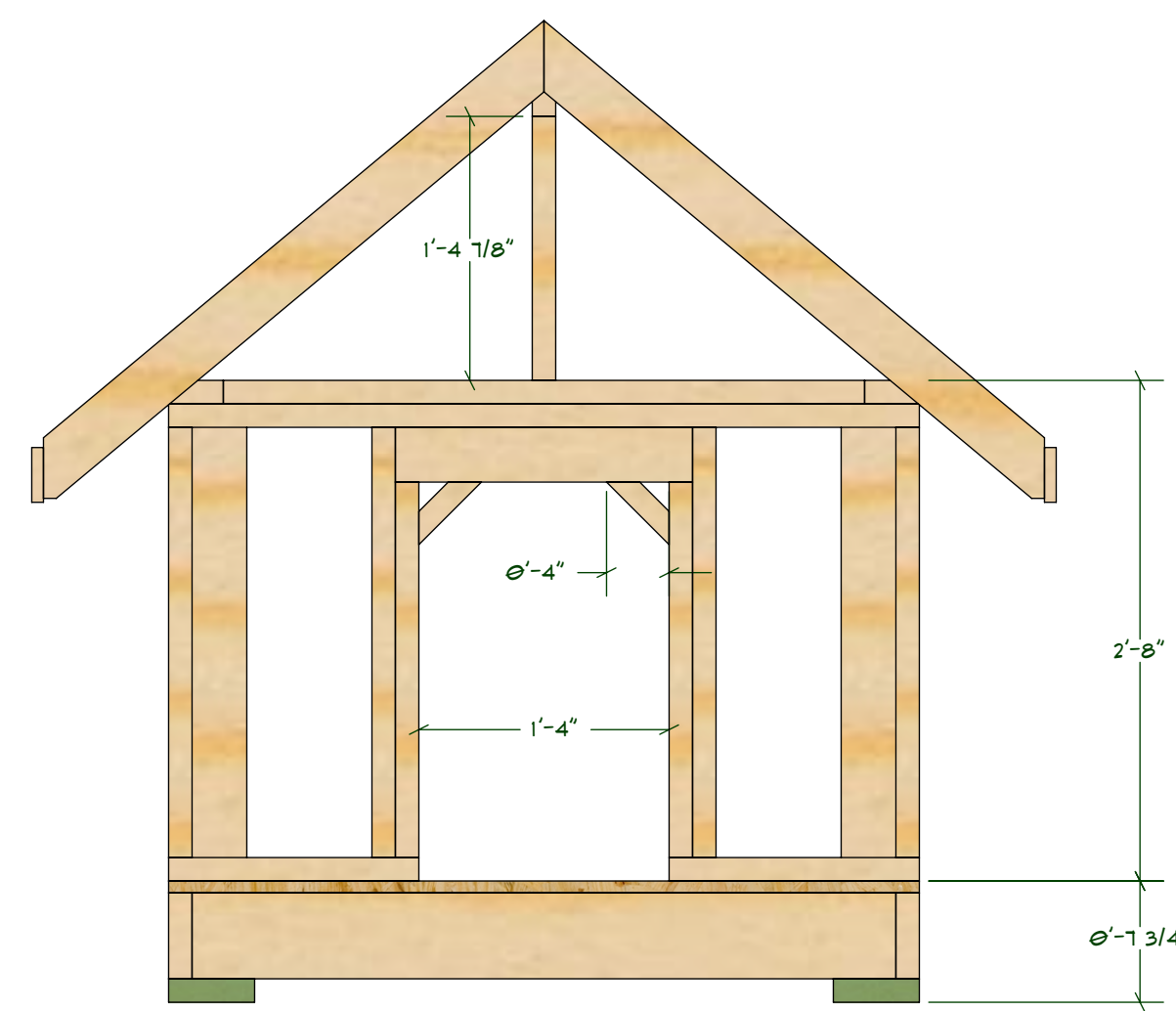
FRONT WALL FRAMING
