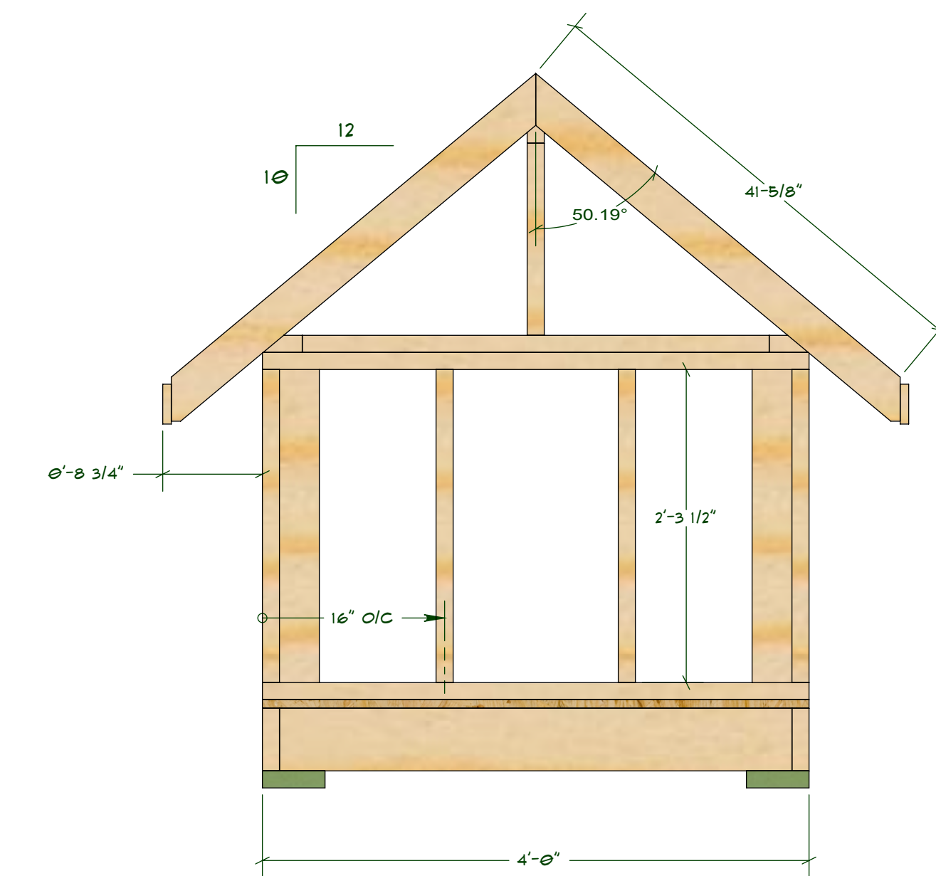
REAR WALL FRAMING
