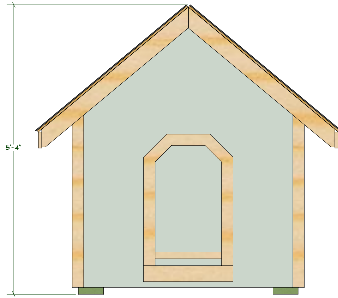
FRONT ELEVATION
