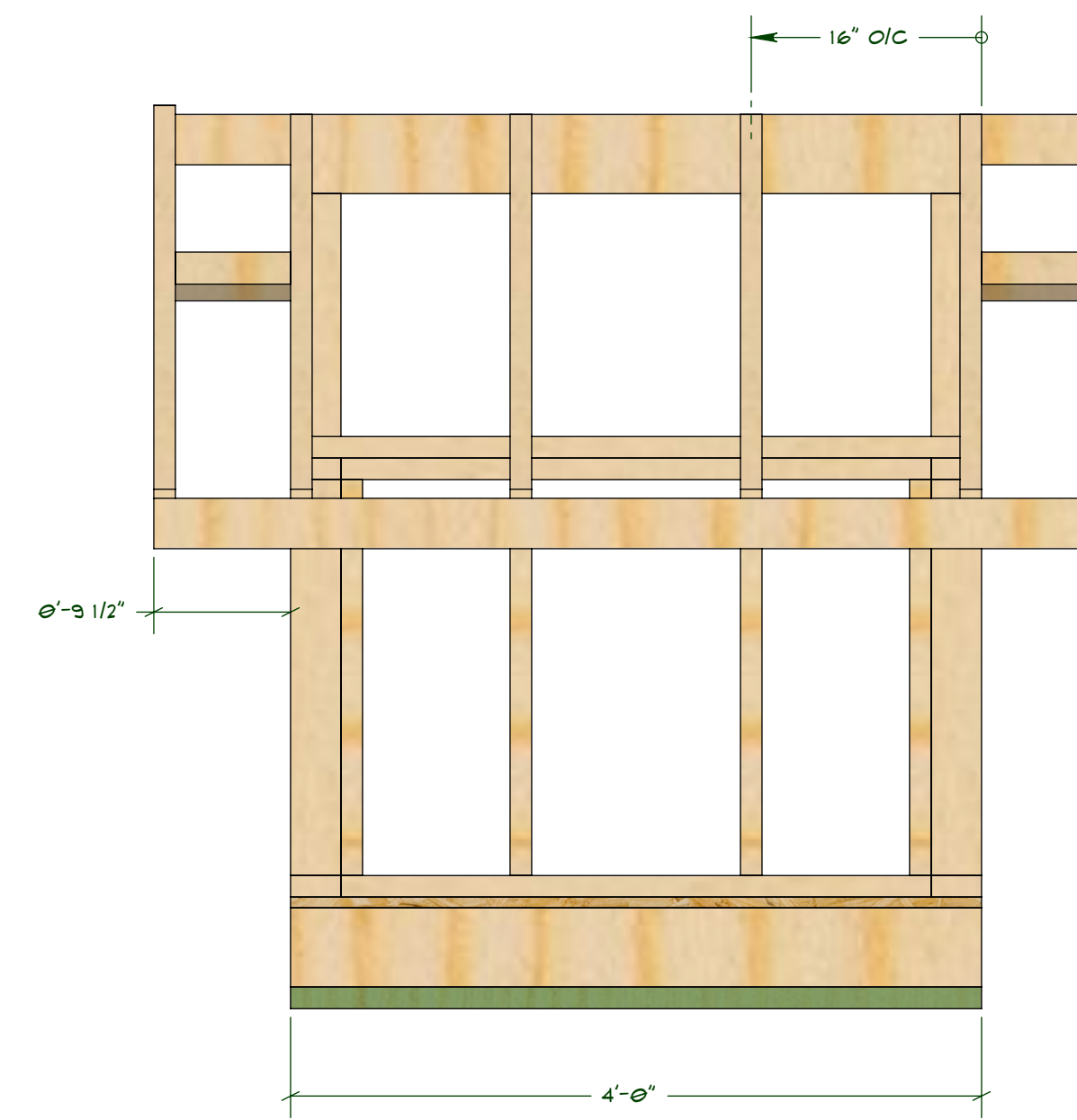
SIDE WALL FRAMING
