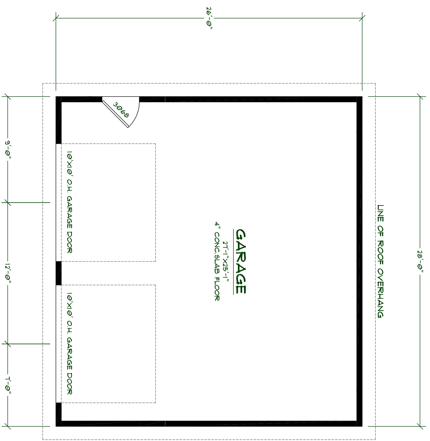
FLOOR PLAN
