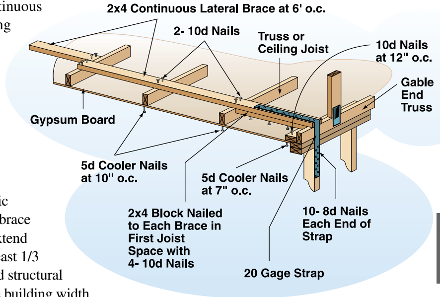
Figure 11. Ceiling Bracing Gable Endwall
