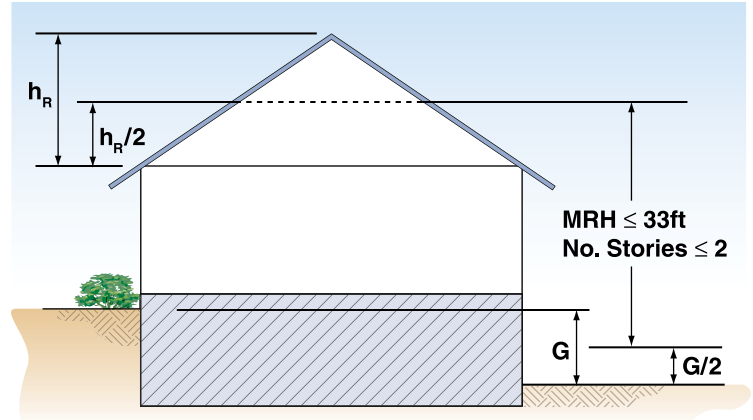
Figure 2. Mean Roof Height (MRH)
