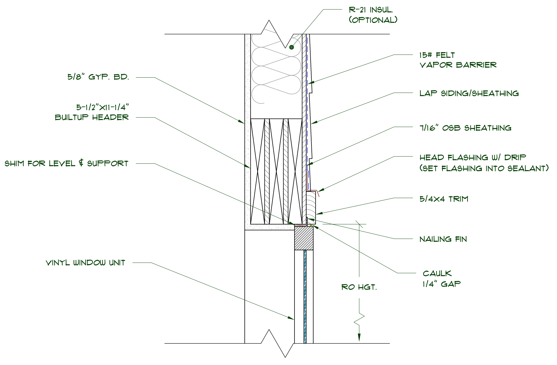
4 WINDOW HEAD DETAIL SCALE: 2"=1'-0"
