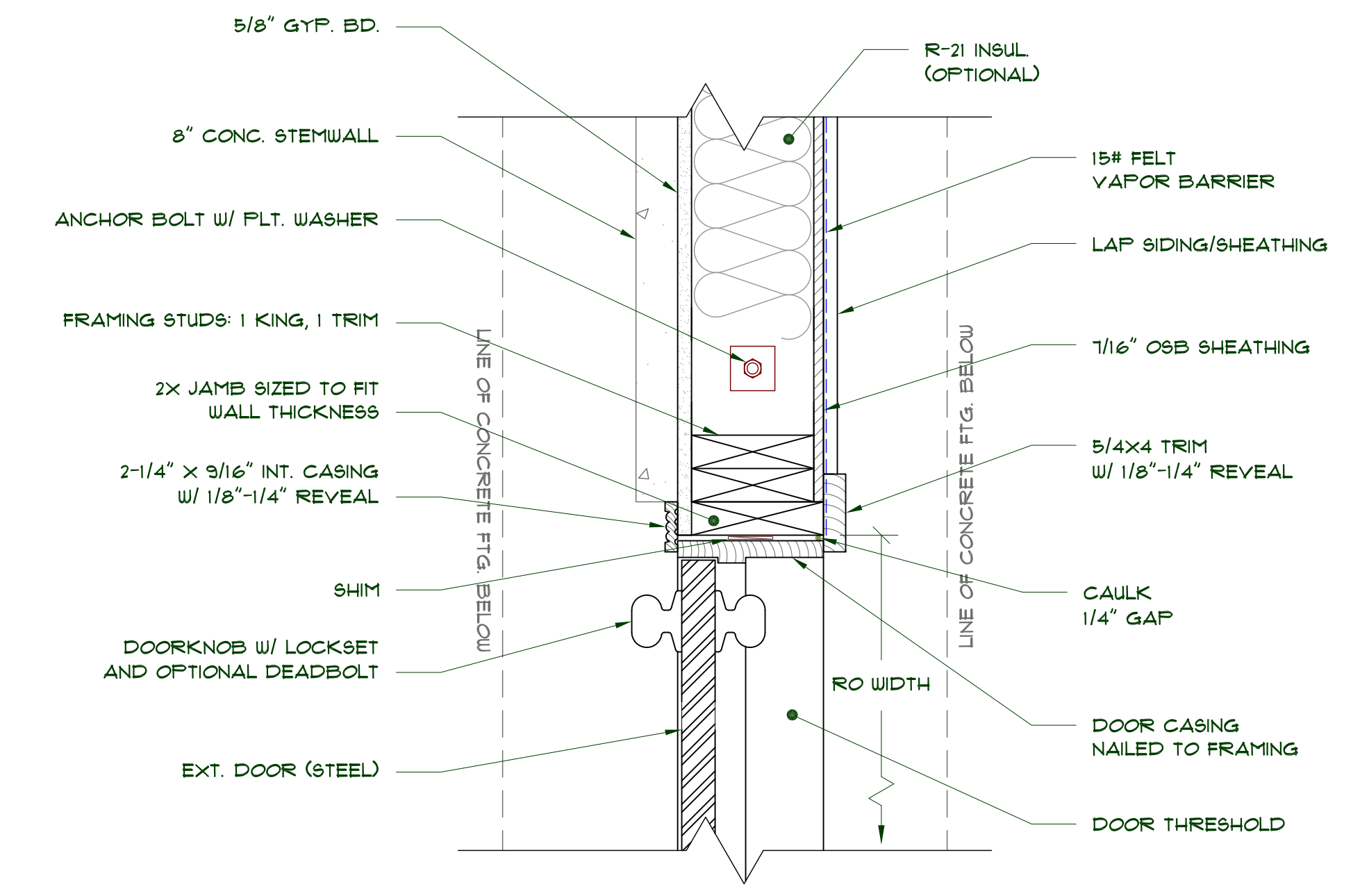
3 DOOR JAMB DETAIL SCALE: 2"=1'-0"
