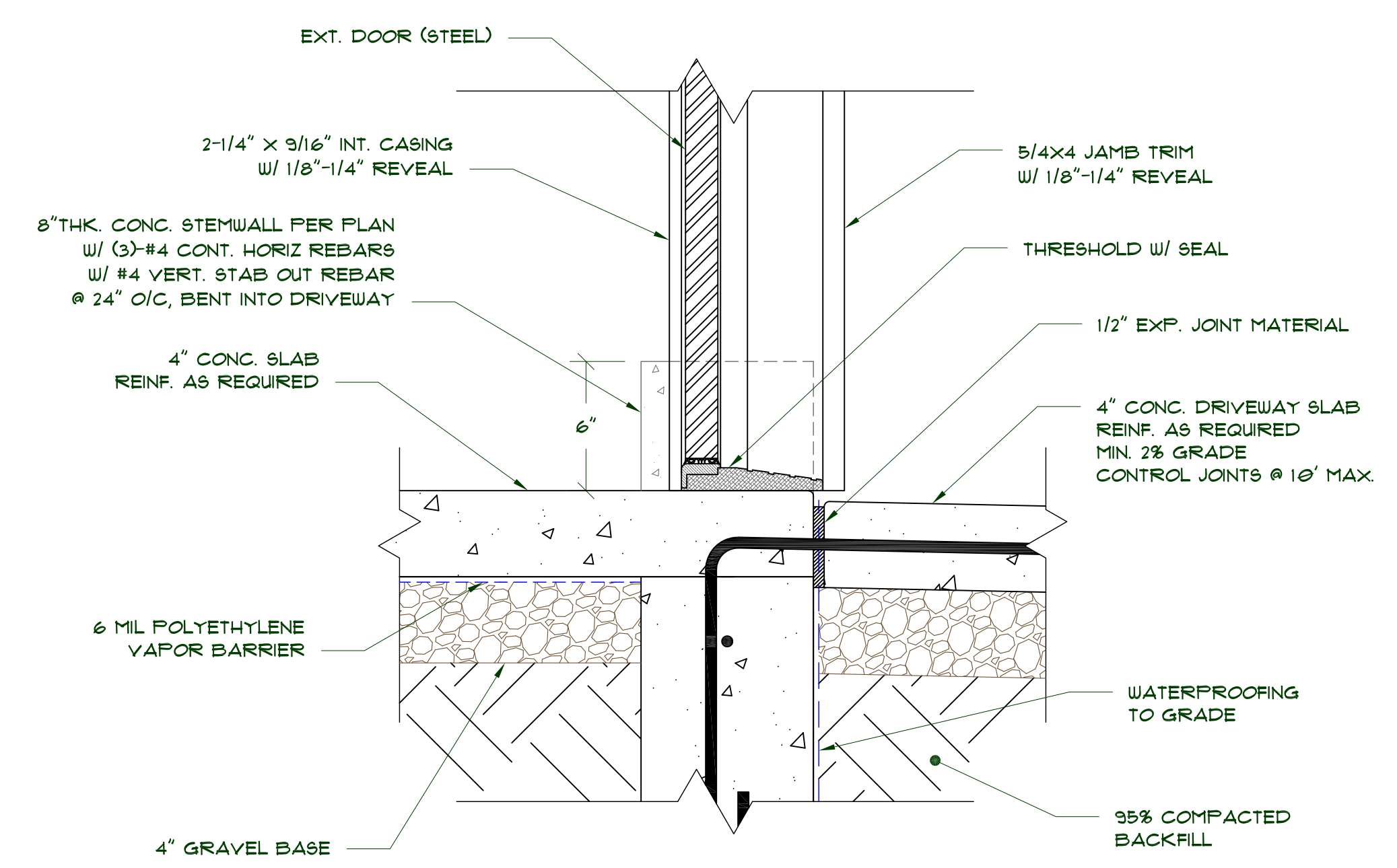
2 DOOR THRESHOLD DETAIL SCALE: 2"=1'-0"
