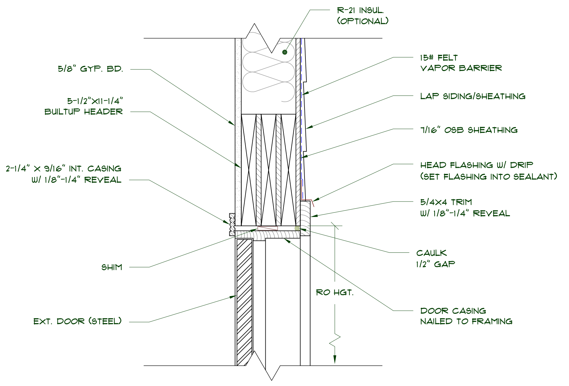
1 DOOR HEAD DETAIL SCALE: 2"=1'-0"
