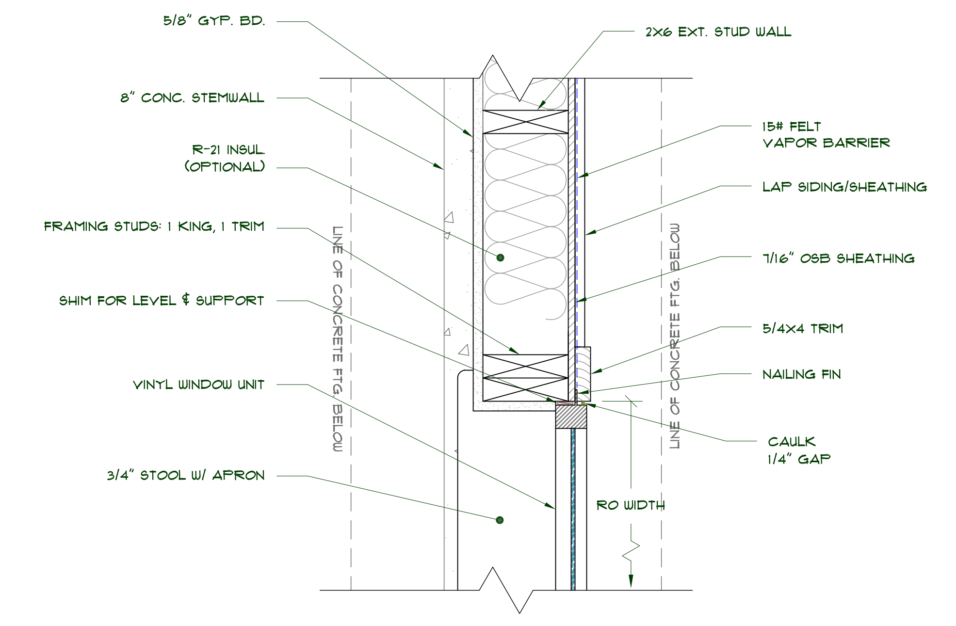
6 WINDOW JAMB DETAIL SCALE: 2"=1'-0"
