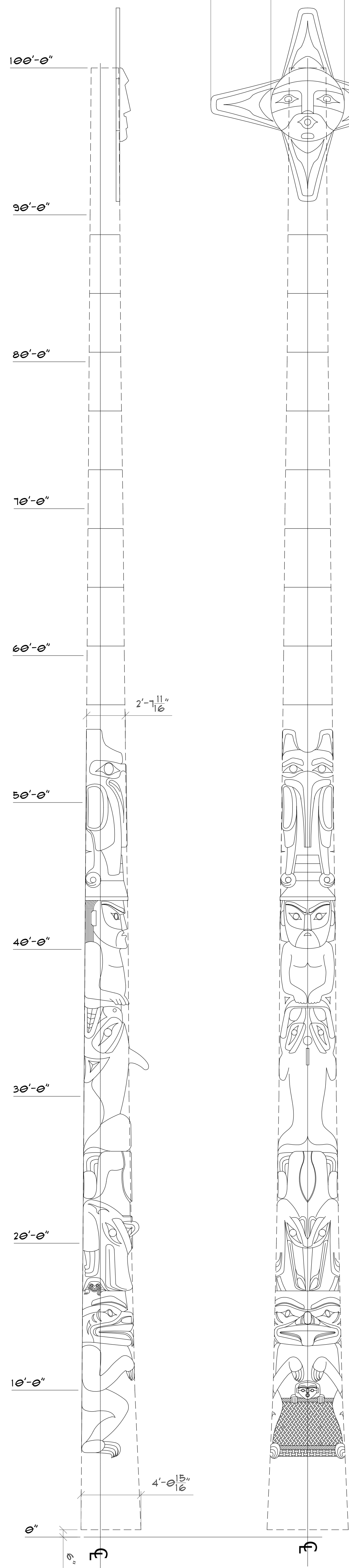
POLE ELEVATIONS SCALE: 1/4" = 1'-0"
